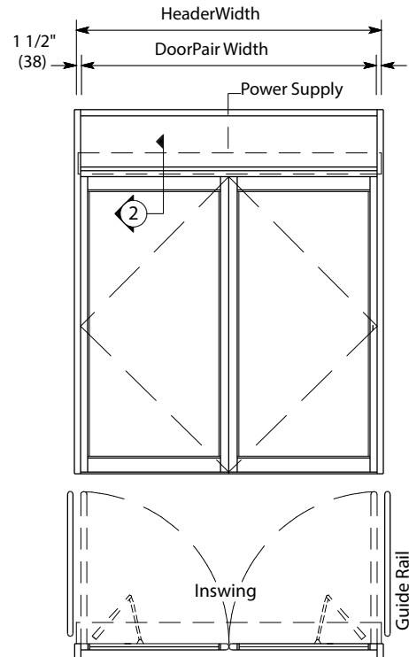
Pair Unit Floor Plan with Elevation
