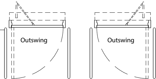
Single Units Floor Plans with Elevations LHR & RHR shown. LH & RH are Inswing
