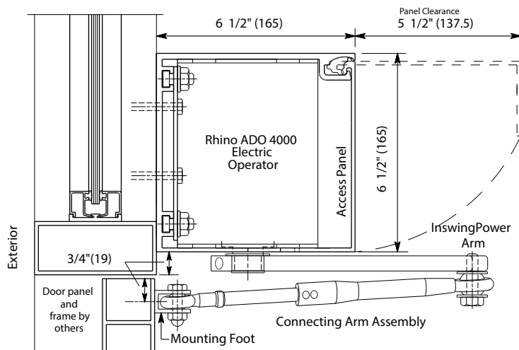
Vertical Section ②
